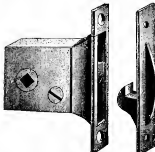
Figs. 2563-2561. Sliding-door Mortise-latch.
